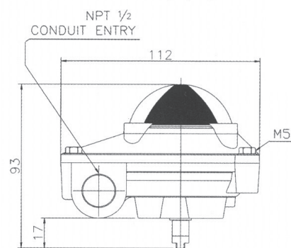
STANDARD NAMUR SHAFT (mm)
