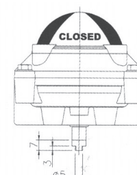
STANDARD NAMUR SHAFT (mm)
