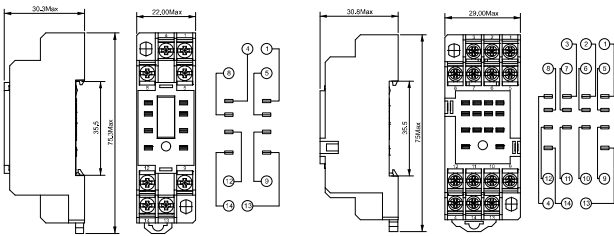
DPYF08A-3
