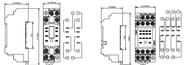
DPYF08A-E3
