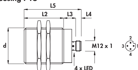
Housing I-15
