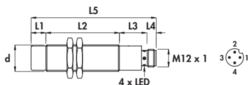
Housing I-12
